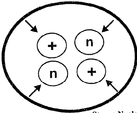
Strong Nuclear Force
