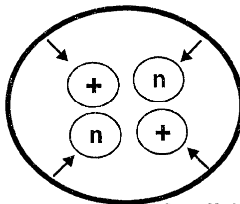
Strong Nuclear Force
