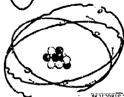
MODEL OF ATOMIC STRUCTURE
