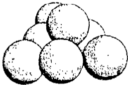
Protons (red marbles) have positive electric charge
