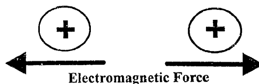
Figure 1.1: The electromagnetic force is attractive for unlike charges, and repulsive for like charges.
