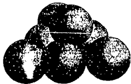
Neutrons (blue marbles) have no electric charge
