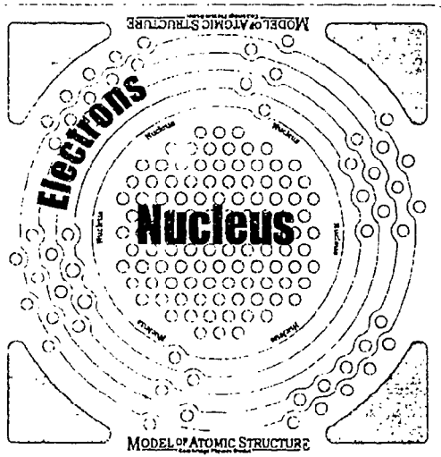
Electrons (yellow marbles) have negative electric charge
